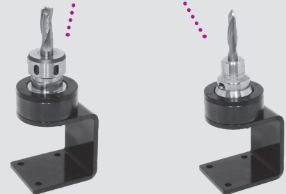
Detail: HSK mounting device for clamping chucks (left) and for the „ps-System“ chuck (right)
